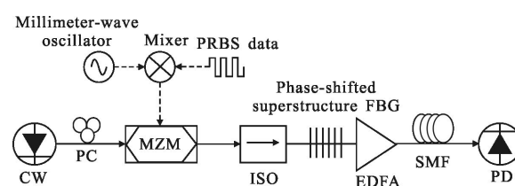
Fig.2 Schematic setup of the OSSB+C RoF system
