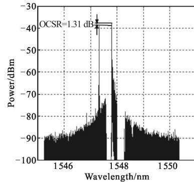
Fig.4 Simulated optical spectrum of OSSB
