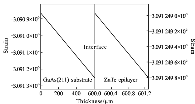
(a) 延[1-1-1]方向 (a) Along [1-1-1]direction
