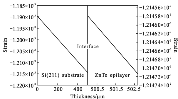
(b) 延[01-1]方向 (b) Along [01-1]direction
