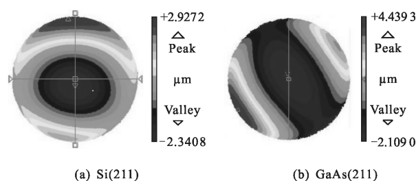
图 1 经过抛光后的衬底表面等高线图 Fig.1 Surface contour maps of polished substrates
