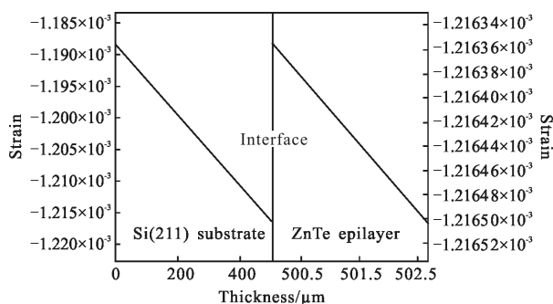
(a) 延[1-1-1]方向 (a) Along [1-1-1]direction
