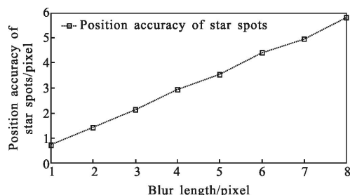
图 14 不同模糊长度时绕非光轴转动对质心提取精度的影响 Fig.14 Influence of cross boresight rotation on star spot centroids with different blur lengths
