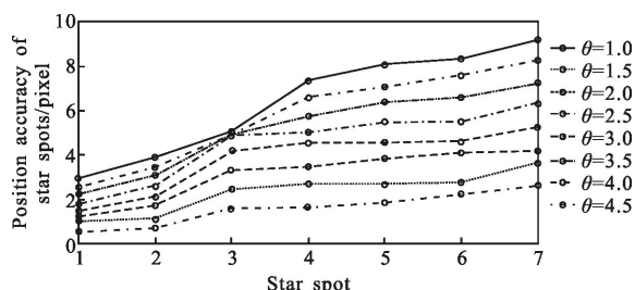
图 15 不同旋转角度的绕光轴转动对质心提取精度的影响 Fig.15 Influence of boresight rotation on star spot centroids with different rotation angles
