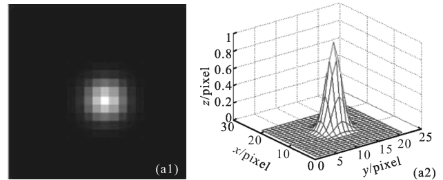
(a) Simulation of single star image
