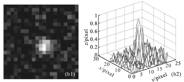
(b) Simulation of single star image with Gaussian noise
