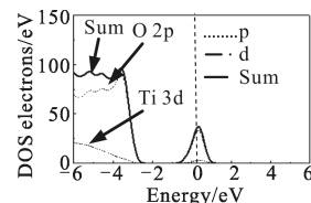
(c) 一个 O 空位表面的态密度 (c) Anatase TiO 2 (101) surface with an oxygen vacancy density of states
