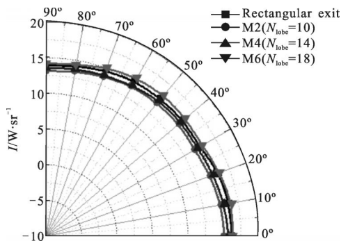
图11 水平面上,整体红外辐射强度分布(不同波瓣数) Fig.11 Horizontal infrared radiation intensity(3~5 μm) for IR suppressors of different mixing duct lobe numbers
