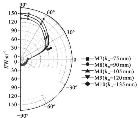
图13 垂直平面上,整体红外辐射强度(不同瓣高) Fig.13 Effects of mixing duct lobe heights on vertical infrared radiation(3~5 μm) for IR suppressors
