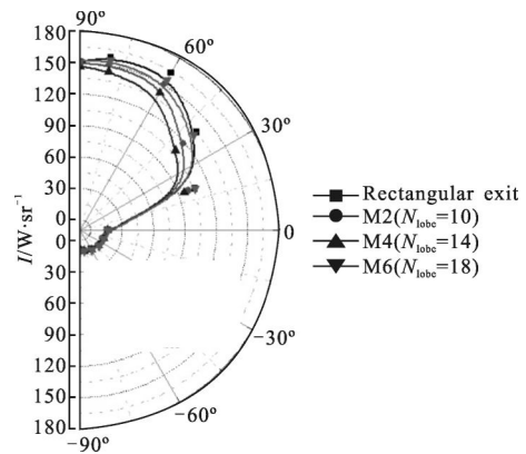
图12 垂直方向,整体红外辐射强度(不同波瓣数) Fig.12 Vertical infrared radiation intensity(3~5 μm) for IR suppressors of different mixing duct lobe numbers
