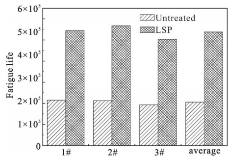
图 6 旋转弯曲疲劳试验数据 Fig.6 Rotary bending fatigue experiment results
