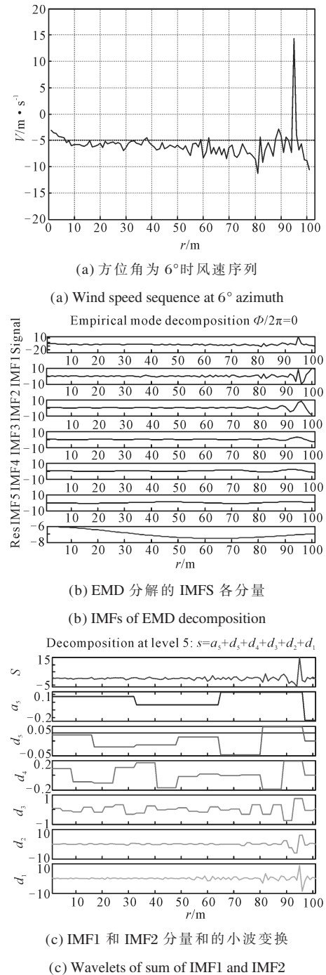
图 3 方位角为 6° 时风速序列、EMD 分解和小波分解示意图 Fig.3 Wind speed sequence, decomposition of EMD and wavelets at 6° azimuth
