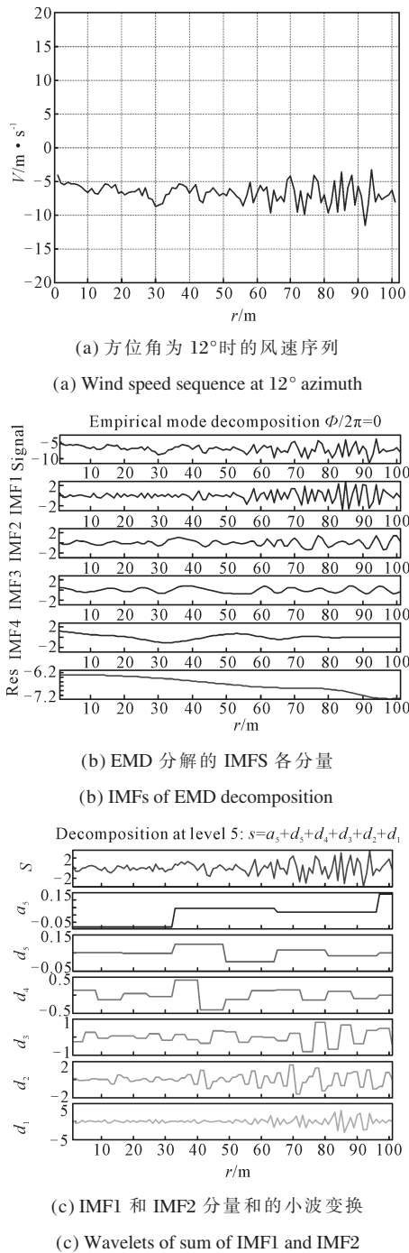
图 2 方位角为 12° 时风速序列、EMD 分解和小波分解示意图 Fig.2 Wind speed sequence, decomposition of EMD and wavelets at 12° azimuth
