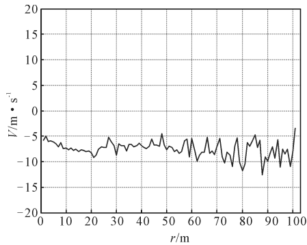
(a) 方位角为 24^\circ 时风速序列 (a) Wind speed sequence at 24^\circ azimuth
