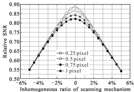
图 4 扫描非均匀性对探测不同尺度目标性能的影响 Fig.4 Effect of scanning inhomogeneous on detecting performance of target scales
