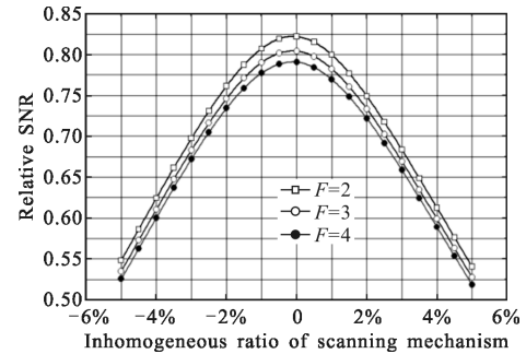
图 5 扫描非均匀性对不同 F 数光学系统探测性能的影响 Fig.5 Effect of scanning inhomogeneous on detecting performance of different F number optical systems
