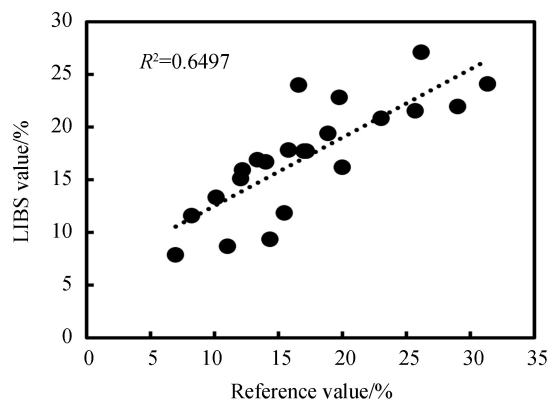
(b) Delay time: 500 ns
