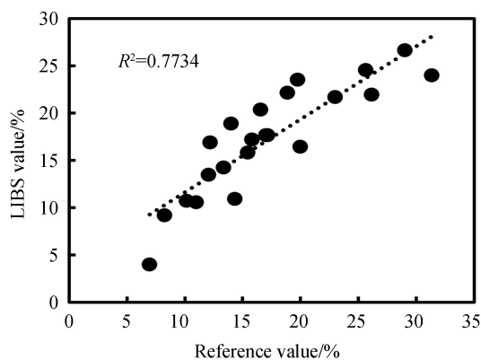
(a) Delay time: 250 ns
