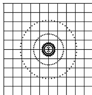
(a) Spot diagram of spherical lens
