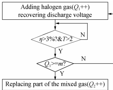
Fig. 4 The work flow diagram of adding halogen gas
