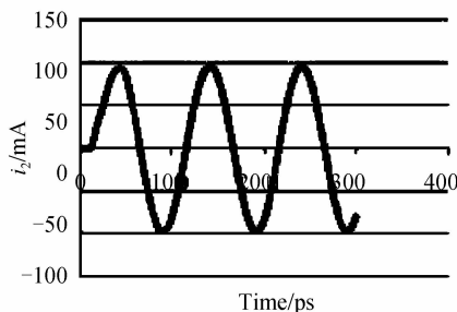
(b) Second branch current
