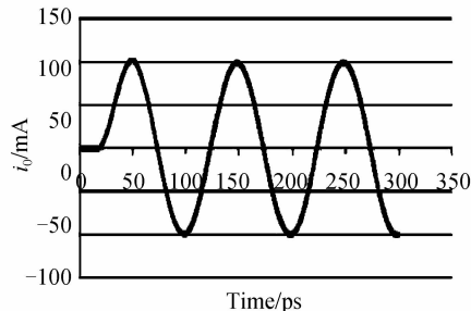
(c) Combining output
