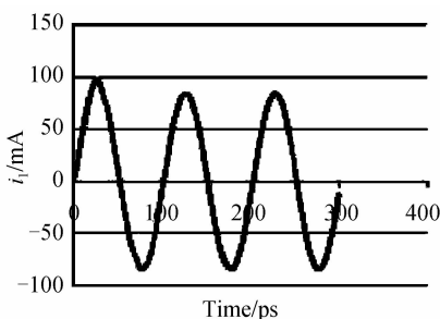
(a) First branch current
