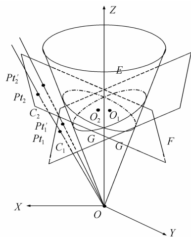
图 4 斜圆锥坐标系下由图像特征恢复空间目标 Fig. 4 Spatial targets from image features in oblique cone coordinates
