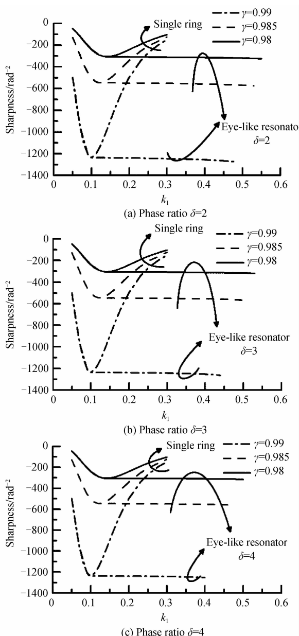
图5 Fano 谐振峰的尖锐度与外环场强耦合系数 k_1 关系图 Fig. 5 The relationship of sharpness and the outer loop coupling coefficient k_1
