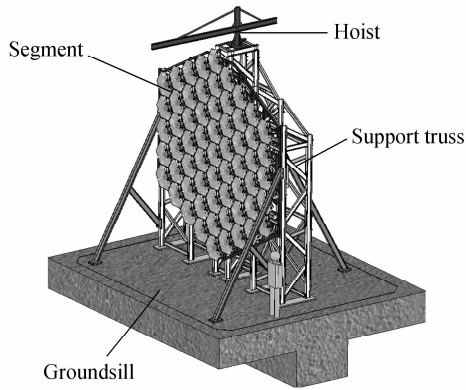
图 1 拼接主镜三维效果图 Fig. 1 3D view of segmented mirror
