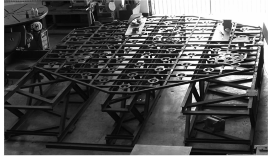
图 3 车间装配中的支撑桁架 Fig. 3 Support truss at work shop
