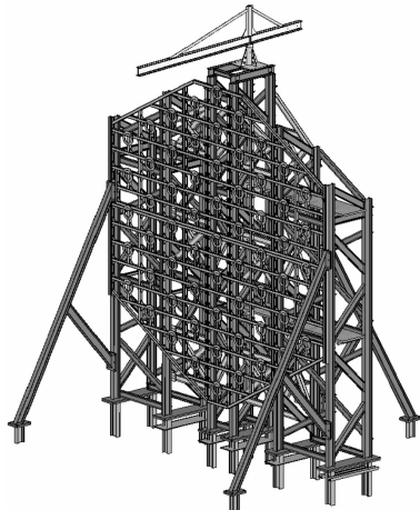
图 2 支撑桁架三维效果图 Fig. 2 3D view of support truss
