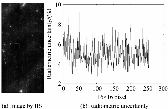
图10 干涉成像光谱仪的光谱辐亮度不确定度检测 Fig. 10 Radiometric uncertainty of Interference Imaging Spectrometer on-orbit evaluating
