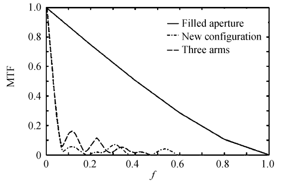
(b) The direction of minimal MTF( F=10\% )
