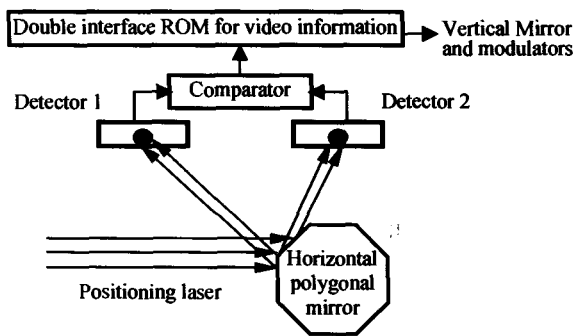
图 4 转镜实时定位系统新方案示意图 Fig. 4 Schematic diagram of real-time positional system for horizontal polygonal mirror
