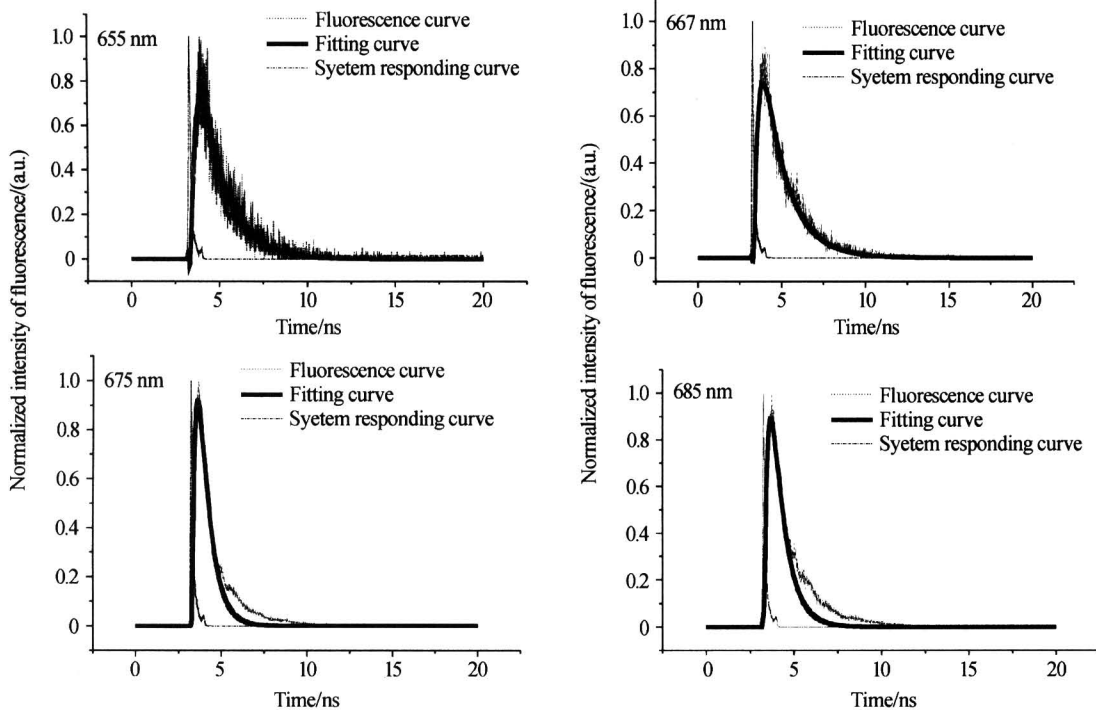
Fig. 3 Time resolved fluorescence spectra of LHC II excited by 630nm measured at different waveband
