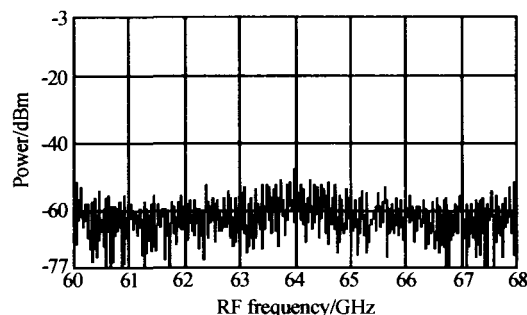
Fig. 4 RF spectrum of the recovered clock
