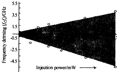
Fig. 6 Locking range as a function of the injected power
