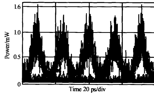
Fig. 8 Eye diagram of the transmitted PRBS signal
