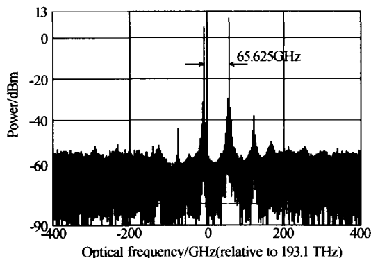
Fig. 2 Optical spectrum of the free-running state
