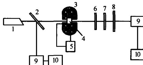
1. KDP adjust QNd:YAG laser; 2. Beam splitter; 3. Heater furnace; 4. Sample; 5. Temperature controller; 6. Reflector; 7. Green glass; 8. 0.53 μm interfere filter; 9. Power detector; 10. Check up current meter
