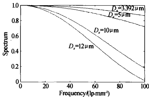
图 3 不同直径针孔的归一化频谱 Fig. 3 Normalized frequency spectrum of pinhole with varies diameters
