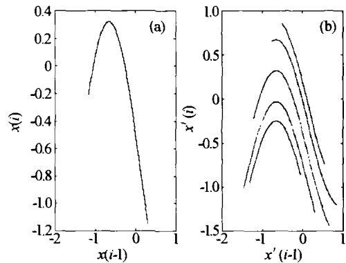
图4 声光双稳态系统混沌反控制的相空间延迟重构 Fig. 4 Phase space delayed reconfiguration of AOB system chaos anti-control
