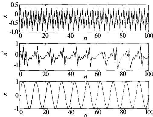
图1 声光双稳态系统混沌反控制输出序列 Fig. 1 Time series of acousto-optic bistable(AOB) system chaos anti-control
