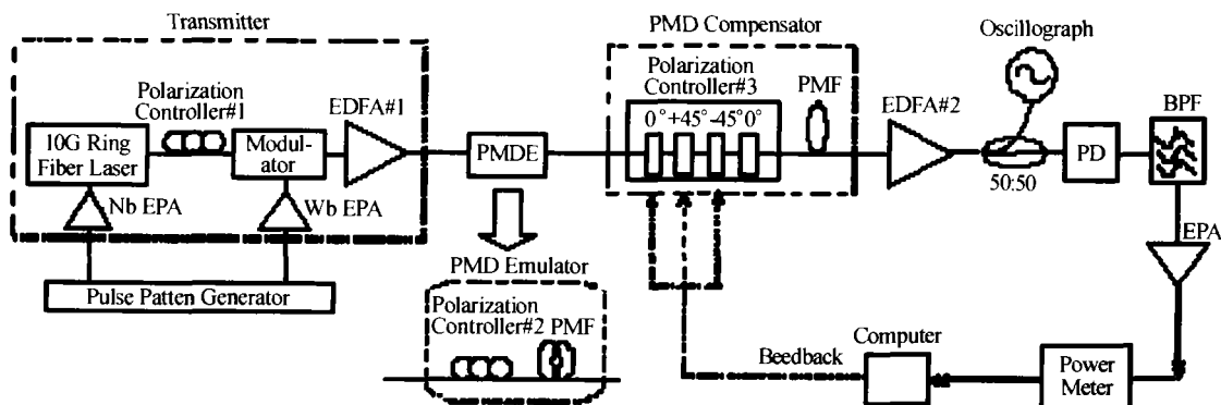
PMDE:PMD Emulator PMF:Polarization Mode Fiber PD:Photonic Detector BPF:Band Pass Filter EPA:Electronic Power Amplifier Wb:Wideband Nb:Narrowband
