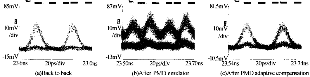
图 6 PMD 自适应补偿实验结果眼图 Fig. 6 The eye diagrams of PMD adaptive compensation experimental result
