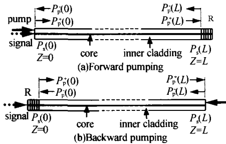
Fig. 2 Schematic illustration of the DCFA with fiber Bragg grating as pump power reflector
