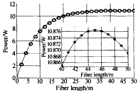
Fig. 7 Signal amplification for EY801 DCFA with different fiber lengths with Bragg reflector for backward pumping
