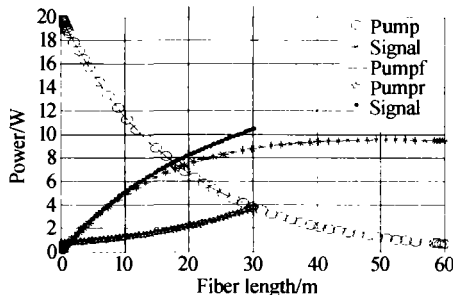
Fig. 3 Signal amplification and pump attenuation along the fiber for EY801 DCFA without Bragg reflector for forward pumping
