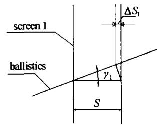
图4 弹道不垂直光幕 Fig. 4 The ballistic is not perpendicular to light screen
