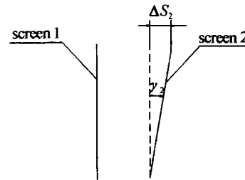
图5 两光幕不平行 Fig. 5 Two light screens are not parallel
