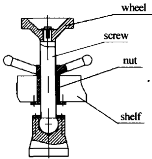
图3 地脚 Fig. 3 The support screw
