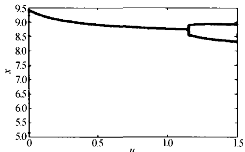
图4 周期2的倍周期分岔延迟控制( A=0.46 ) Fig. 4 Control of delaying period-doubling bifurcations (2p) ( A=0.46 )
