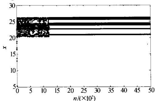
图7 6p周期轨道( A=0.70, B=0.99 )
