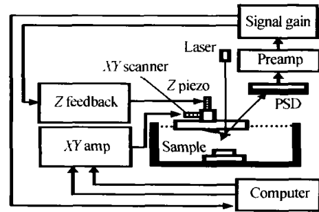
图4 液相型AFM的系统框图 Fig. 4 Schematic diagram of the AFM system measuring in liquid
