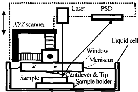
图2 液相探头 Fig. 2 Detector measuring in liquid
