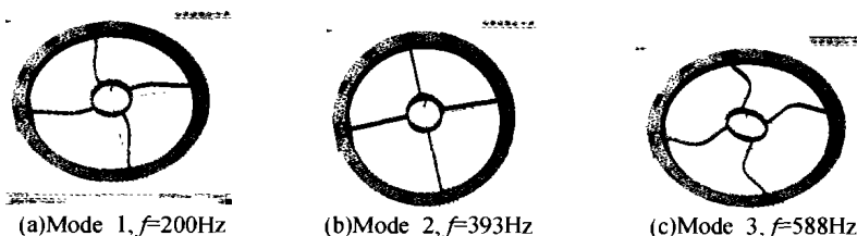
图5 结构2前三阶模态 Fig.5 The first three modes of structure 2
