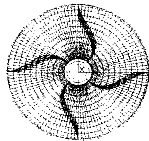
图4 结构1的1阶模态 Fig.4 The first mode of structure 1
