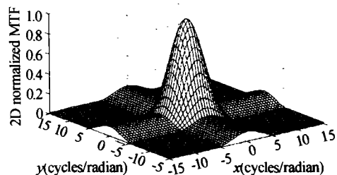
图 3 10.6 \mu\text{m} 激光雷达成像的气溶胶 MTF Fig. 3 Aerosol MTF of 10.6 \mu\text{m} imaging Lidar
