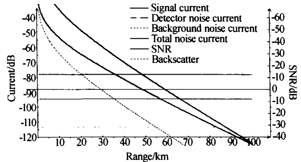
图 2 1.543 \mu\text{m} 直接探测系统在多云天气下性能图 Fig. 2 Performance of 1.543 \mu\text{m} direct detection system under cloudy weather
