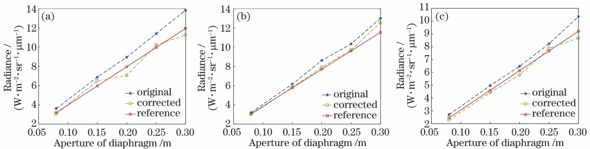
图 8 辐亮度反演结果。(a) 谱段 R; (b) 谱段 G; (c) 谱段 B Fig. 8 Radiance inversion results. (a) Red; (b) green; (c) blue
