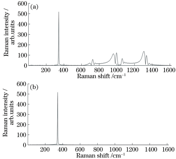
图 11 0 视场杂散光抑制前后的光谱。(a)抑制前;(b)抑制后 Fig. 11 Raman spectra before and after stray light control in 0° FOV. (a) Before control; (b) after control
