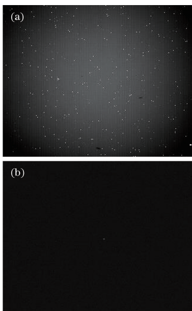
图 2 (a)原始图像;(b)两点校正后的恒星图像 Fig. 2 (a) Original image; (b) stellar image after two-point correction
