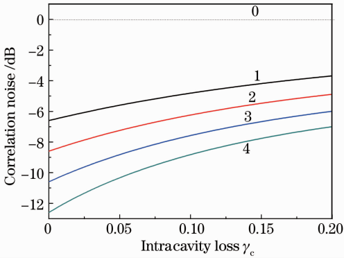
图 3 NOPA 输出场关联噪声随内腔损耗的变化 Fig. 3 Dependence of correlation noise of output field of NOPA on intracavity loss
