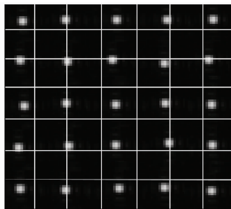
图 2 传统夏克-哈特曼波前传感器图像分割 Fig. 2 Picture segmentation of conventional Shack-Hartmann wavefront sensor
