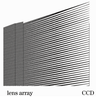
图 7 光线追迹结果(点光源距 SHWS 为 200 \text{ mm} ) Fig. 7 Result of ray trace (distance between point source and SHWS is 200 \text{ mm} )
