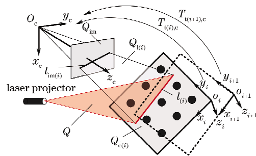
图 2 结构光视觉传感器标定过程示意图 Fig.2 Calibration process of structured light vision sensor
