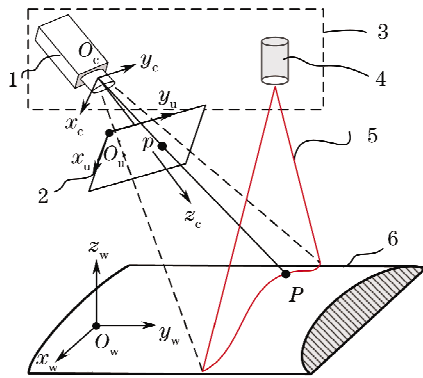
图 1 线结构光视觉传感器模型的几何结构关系图 Fig.1 Geometric structure of line structured light vision sensor model
