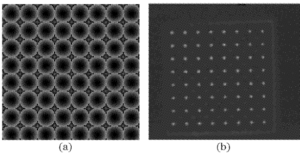
图 4 (a) 8 \times 8 透镜阵列与 (b) 光斑阵列 Fig. 4 (a) Driving pattern of the 8 \times 8 lenslet array on the LCTV, (b) detected 8 \times 8 spot array
