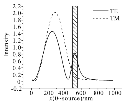
Fig. 8 Intensity profile along x through 50 nm thickness Au film at 100 nm wide aperture for TM and TE mode
