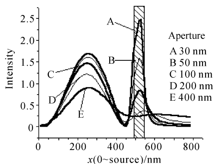
Fig. 7 Intensity profile along x through Au film 50 nm thick with different aperture at the center for TM mode
