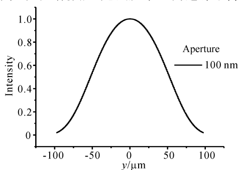
Fig. 3 The intensity profile of the base mode of the resonator with aperture 100 nm wide
