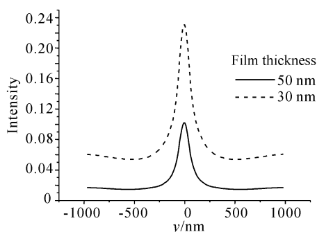
Fig. 6 Intensity profiles along y of the output through the 100 nm wide aperture with different thickness for TE mode
