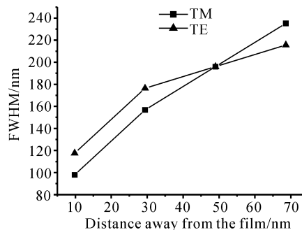
Fig. 9 The spot size (FWHM) as a function of the distance away from the film for TM and TE mode (thickness: 50 nm, aperture: 100 nm)
