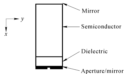
Fig. 1 The detail of the VSAL
