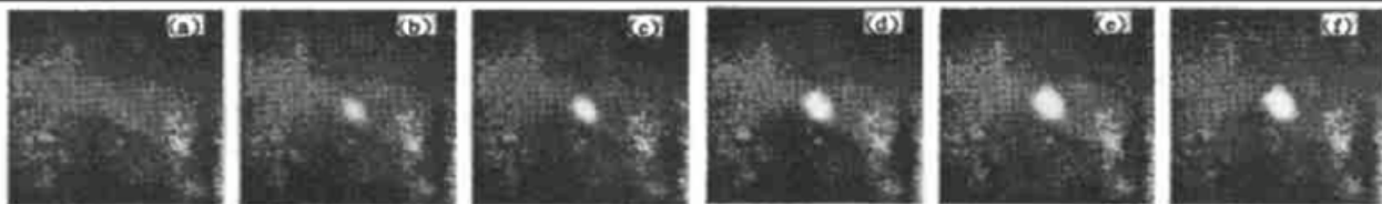
Fig. 2 CCD photos of laser trapped rubidium atoms. The light area in middle of each photo is the trapped atoms, (a) to (f) correspond a successive increase of the gradient of magnetic field. (a) 0.0005 T/cm; (b) 0.0007 T/cm; (c) 0.0009 T/cm; (d) 0.0011 T/cm; (e) 0.0014 T/cm; (f) 0.0016 T/cm
