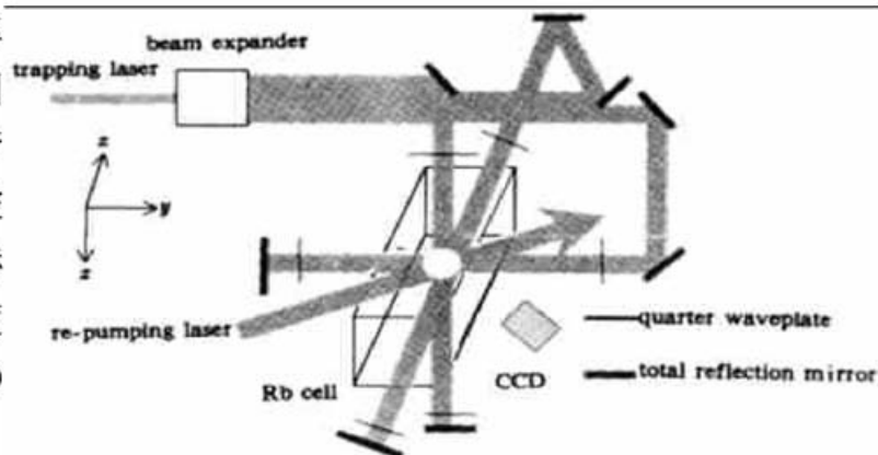
Fig. 1 Setup of laser cooling and trapping of rubidium atoms
