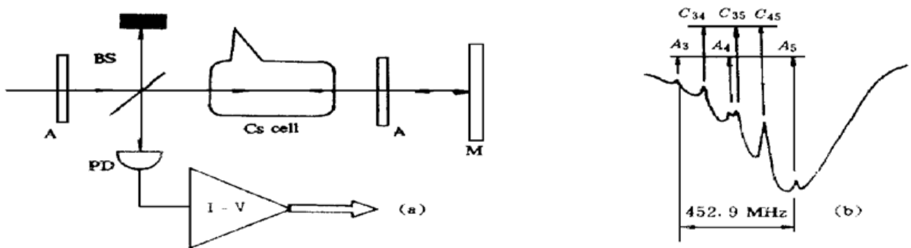
Fig. 2 (a) Sketch of the saturated-absorption spectroscopy of cesium atoms. A: neutral attenuators; BS: beam splitter; Cs cell: saturated vapour cell of cesium atoms; M: high-reflectivity mirror; PD: photo-diode detector; I-V: I-V converter. (b) The saturated-absorption spectroscopy of cesium atoms with a Doppler background ( D_2 line of cesium atoms: 6^2S_{1/2}F = 4 - 6^2P_{3/2}F' = 3, 4, 5 transition)
