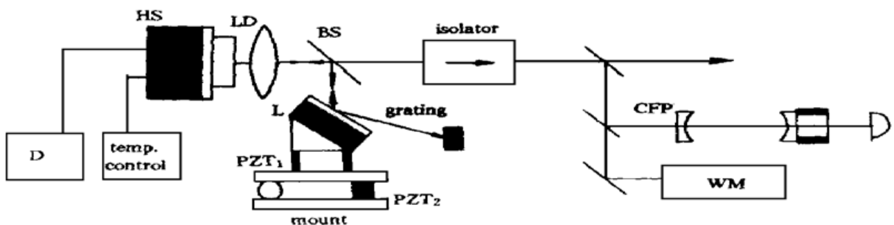
Fig. 1 Schematic of the experimental setup. LD: single-mode GaAlAs semiconductor laser; HS: heat sink; D: constant-current driver; temp. control: high-stability temperature controller; L: collimating lenses assembly; BS: beam splitter; isolator: optical isolator; grating: 1200 grooves/mm blazed grating; PZT 1 : ring piezo transducer; PZT 2 : piezo transducing plate; mount: two-dimension high-resolution mirror mount; CFP: scanning confocal F-P cavity; WM: wavelength meter
