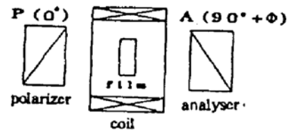
Fig. 1 Measuring cell
