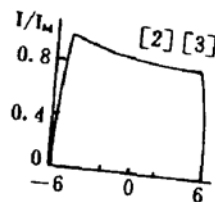
Fig. 2 The nearfield distribution of light intensity (The cross section at near field centre [2,3] . O—the mirror centre)
