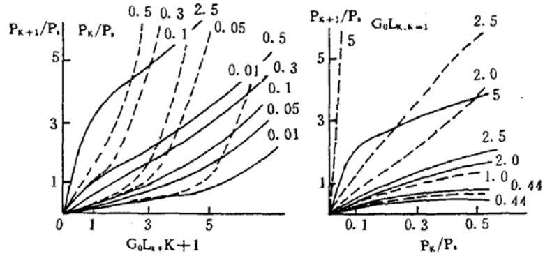
Fig. 15 (P_{K+1}/P_s), (P_K/P_s) \sim G_0 L_{K,K+1} , (P_{K+1}/P_s, (G_0 L_{K,K+1}) \sim P_K/P_s
