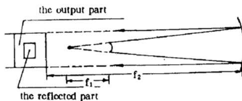
Fig. 1 The positive branch confocal unstable cavity
