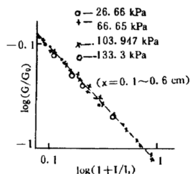
Fig. 4 \log(1 + I/I_s) \sim \log(G/G_0) [4]
