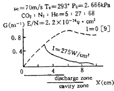
Fig. 12 G_0, G, I \sim X
