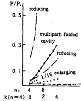
Fig. 18 The output power of the multi-path folded cavity comparing with that of the amplifier in which the laser beam are duced and enlarged
