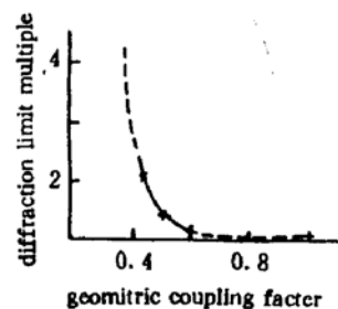
Fig. 3 Geometric coupling factor ~ diffraction limit multiple
