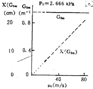
Fig. 11 X(G_{0m}), G_{0m} \sim u_0 u_0 — flow velocity
