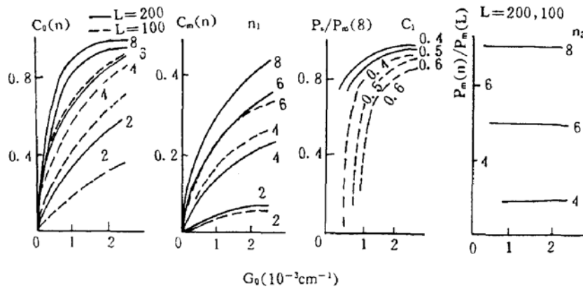
Fig. 8 C_0(n, L), C_m(n, L), \frac{P_s}{P_m(S)}(c), \frac{P_m(a)}{P_m(2)}, \sim G_0
