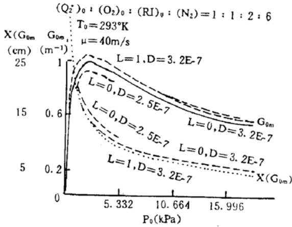
Fig. 10 X(G_{0m}), G_{0m}, (L, D) \sim P_0 G_{0m} — optimum small signal gain, X(G_{0m}) — the position of G_{0m} , P_0 — pressure
