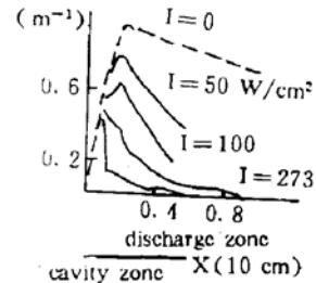
Fig. 13 G_0, G, I \sim X
