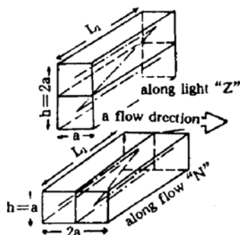
Fig. 5 The light paths in the 3 paths folded cavity
