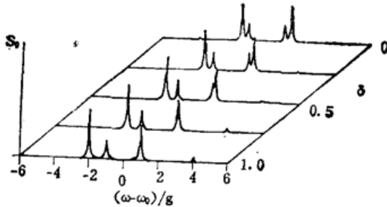
Fig. 1 Emission spectrum of atoms in vacuum field versus \delta (=g_a/g)
