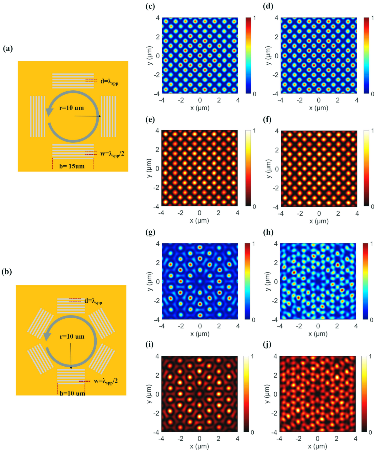
Fig. 5. (a),(b) Quadrilateral and hexagonal gratings, respectively. The blue circular arrow represents the polarization direction of the excitation light, which is left circular polarized. (c),(d) Left circular polarized and right circular polarized components of the SPP field generated by the quadrilateral grating under the left circular polarized excitation light. (e),(f) The corresponding nonlinear signals generated under the right and left circular polarized pump lights. (g)-(j) The corresponding results for the hexagonal grating.
