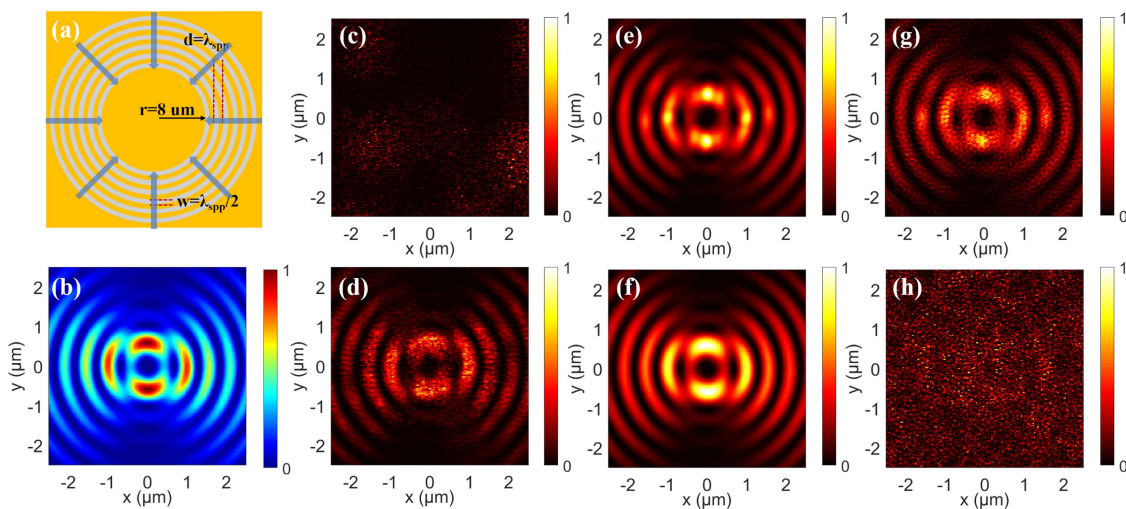
Fig. 2. (a) Schematic of the grating structure used to excite the SPP. The arrow (blue) represents the polarization direction of the excitation light, which is radially polarized. (b) The E_x component of the SPP field generated by the third-order vortex radially polarized light incident on the grating. (c)–(h) The nonlinear signal with the x -polarization pump light when the coefficient is set as (c) 1.2 \times 10^{-4} (m/v) 2 , (d) 10^{-4} (m/v) 2 , (e) 10^{-6} (m/v) 2 , (f) 10^{-7} (m/v) 2 , (g) 10^{-8} (m/v) 2 , and (h) 10^{-9} (m/v) 2 , respectively.
