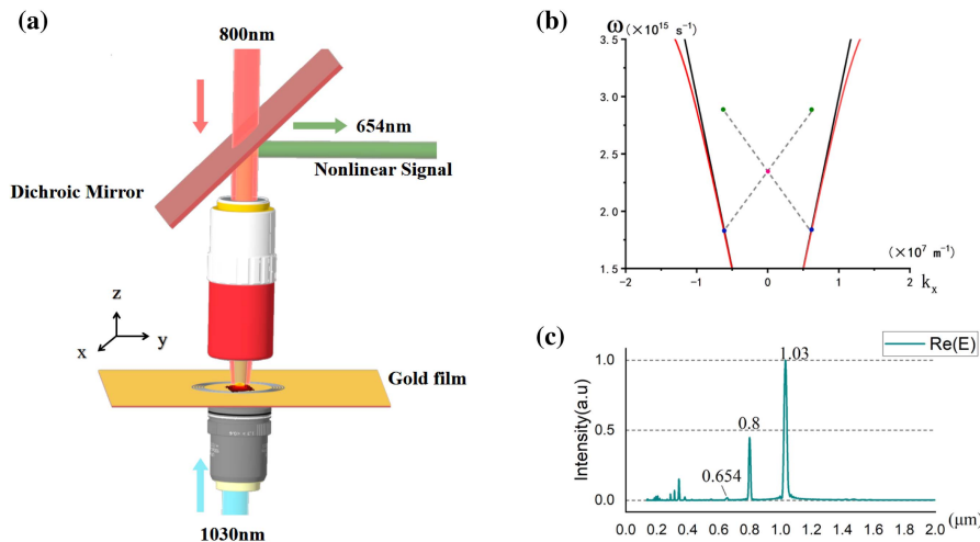
Fig. 1. (a) Schematic diagram of the nonlinear process. (b) Dispersion curve of the SPP on the gold film surface (red line) and the dispersion curve of the photons in vacuum (black line). The pump photon (pink), SPP (blue), and nonlinear photon (green) are connected by dashed lines, which represent the partially degenerate four-wave mixing interaction. (c) Spectrum detected at 5 nm above the gold film in simulation when the FWM happens.
