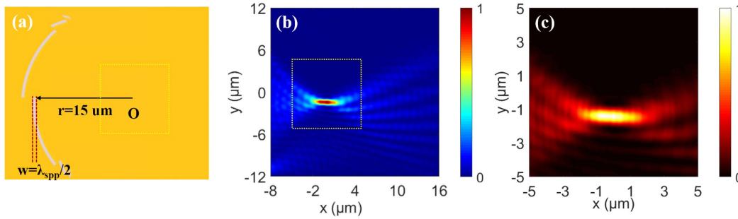
Fig. 4. (a) The structure to generate the PWB is designed based on the principle of the Fourier angle spectrum synthesis. O is the origin of the coordinates. (b) PWB excited under x linearly polarized light. (c) Nonlinear signal [yellow dashed areas in (a) and (b)] obtained under x linearly polarized pump light.
