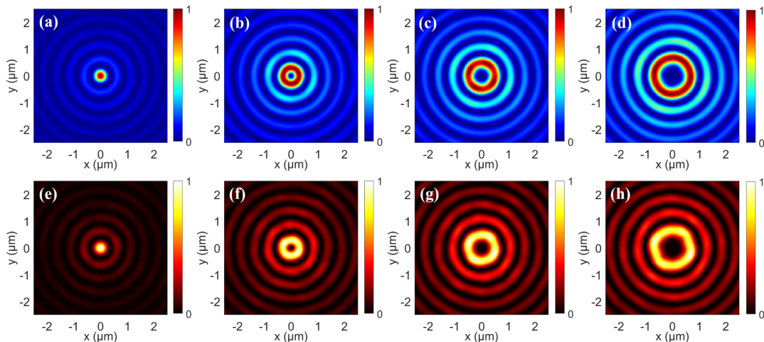
Fig. 3. (a)–(d) Right circular polarized components of the SPP field generated by the radially polarized light of l ( l = 1\text{--}4 ) order vortex incident on the grating. (e)–(h) The nonlinear signals when the pump light is set to right circular polarized.
