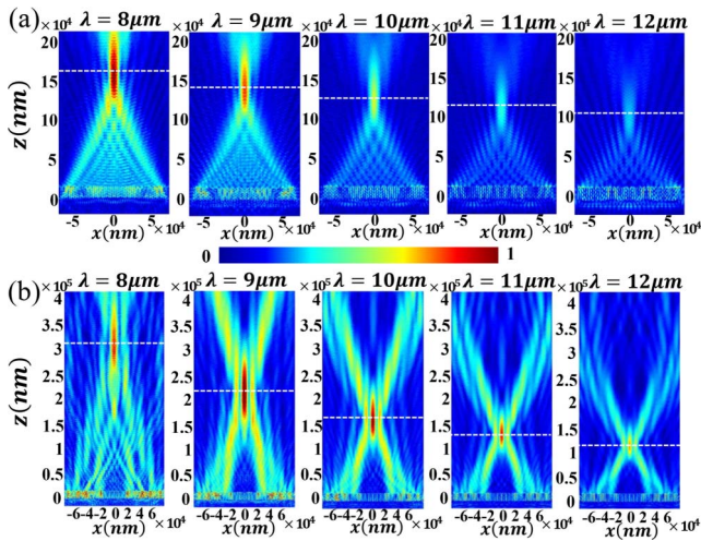
Fig. 5. Simulated ZX slices with the simulated focal length between normal dispersion and the broadband super-chromatic aberration metalems, for the wavelength region ranging from 8 to 12 \mu\text{m} . The focal spot sizes are annotated as dashed white lines. (a) The normal dispersion focal lengths are f = 163, 145, 128, 116, and 107 \mu\text{m} , respectively. (b) The super-chromatic aberration focal lengths are f = 302, 215, 160, 137, and 107 \mu\text{m} , respectively.
