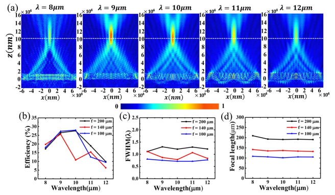
Fig. 3. Performance of broadband achromatic metalens. (a) The simulated ZX slices of the achromatic metalens with a designed focal length f = 100 \mu\text{m} . (b) Operating efficiency. (c) Full width at half-maximum (FWHM). (d) The focal lengths are calculated in the mid-infrared region.
