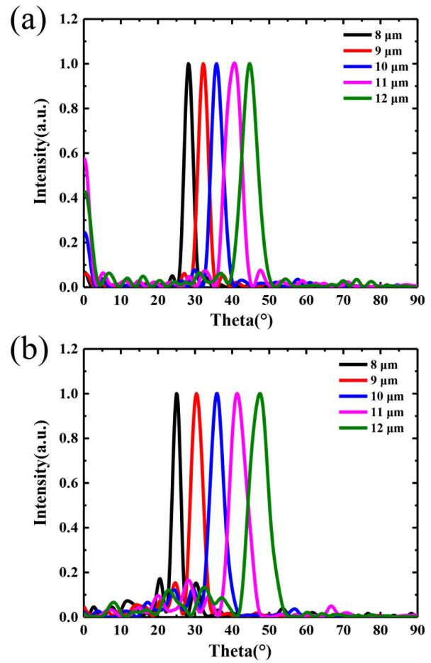
Fig. 6. Contrast between normal dispersion and broadband super-chromatic aberration gradient metalems at various incident wavelength transmission angles. (a) The normal dispersion angle of transmission changes among 28.2^\circ, 32.2^\circ, 35.8^\circ, 40.8^\circ, and 44.8^\circ when the incident wavelength is changed from 8 to 12 \mu\text{m} . (b) The super-chromatic transmission angle changes among 25^\circ, 30.4^\circ, 35.8^\circ, 41.6^\circ, and 47.6^\circ when the incident wavelength is changed from 8 to 12 \mu\text{m} .
