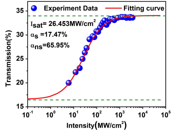
Fig. 2. Saturable absorption characteristics of the \text{MoTe}_2 SA.
