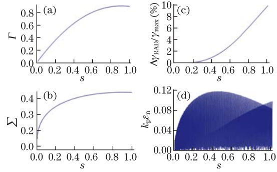
Fig. 8. Numerical solutions of (a) normalized energy \Gamma = \gamma/(2\alpha\chi^2\gamma_g^2/3) , (b) dimensionless beam radius \Sigma , (c) relative radiative energy loss \Delta\gamma_{\text{RAD}}/(2\chi^2\gamma_g^2/3) , and (d) an estimate of the dimensionless normalized emittance given by Eq. (98) over the dephasing length L_{\text{dp}} , i.e., 0 \leq s \leq 1 , for the self-guided bubble regime LPA, a_0 = 4 , n_e = 1.87 \times 10^{16} \text{ cm}^{-3} , \chi = E_{z0}/E_0 = 2 , \alpha = 0.9 , \kappa_{\text{self}} = 1.53 , \gamma_0 = 196 ( W_i = 100 \text{ MeV} ), and \Omega_0 = k_p\varepsilon_{n0}/\gamma_0 = 3 \times 10^{-4} .
