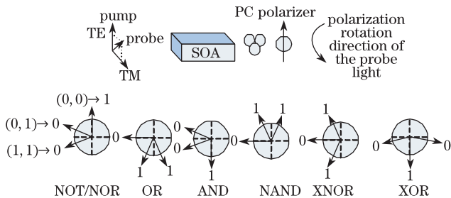
Fig. 1. Schematic of the logic operations based on NPR in a SOA. In the six operations, the arrows represent the polarization states of the probe light existing from the PC, where the bold arrow is the original polarization state without the pump, corresponding to the input state of “00”. The numbers on the arrows represent the operation results.
