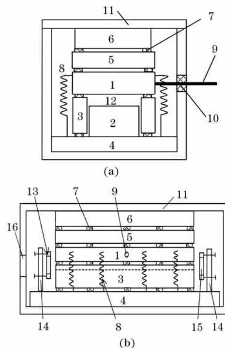
Fig. 1. Transverse (a) and longitudinal (b) cross section diagrams of the slab waveguide laser head. 1: top electrode; 2: bottom electrode; 3: side wall; 4: bearing plate; 5: liner plate; 6: clamp plate; 7: insulating plate; 8: matching inductors; 9: copper electrode link pin; 10: vacuum separation insulation bush; 11: vacuum box; 12: slab waveguide discharge region; 13: convex reflection mirror; 14: mirror mount and adjusting setup; 15: concave reflection mirror; 16: output window.
