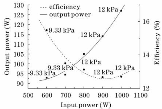
Fig. 2. Laser power output against RF power input.
